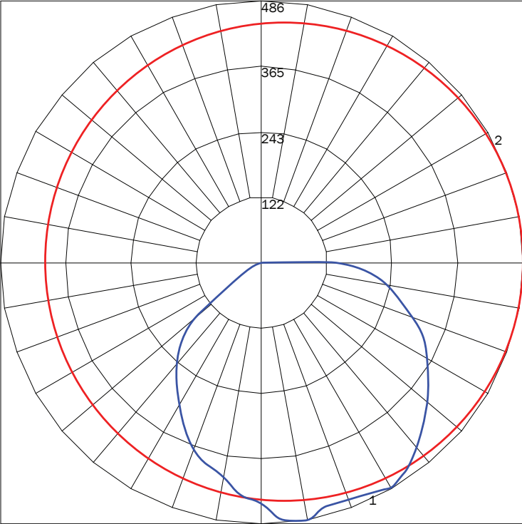
MAXIMUM CANDELA = 486.02 LOCATED AT HORIZONTAL ANGLE = 15, VERTICAL ANGLE = 10 # 1 - VERTICAL PLANE THROUGH HORIZONTAL ANGLES (15 - 195) (THROUGH MAX. CD.) # 2 - HORIZONTAL CONE THROUGH VERTICAL ANGLE (10) (THROUGH MAX. CD.)
