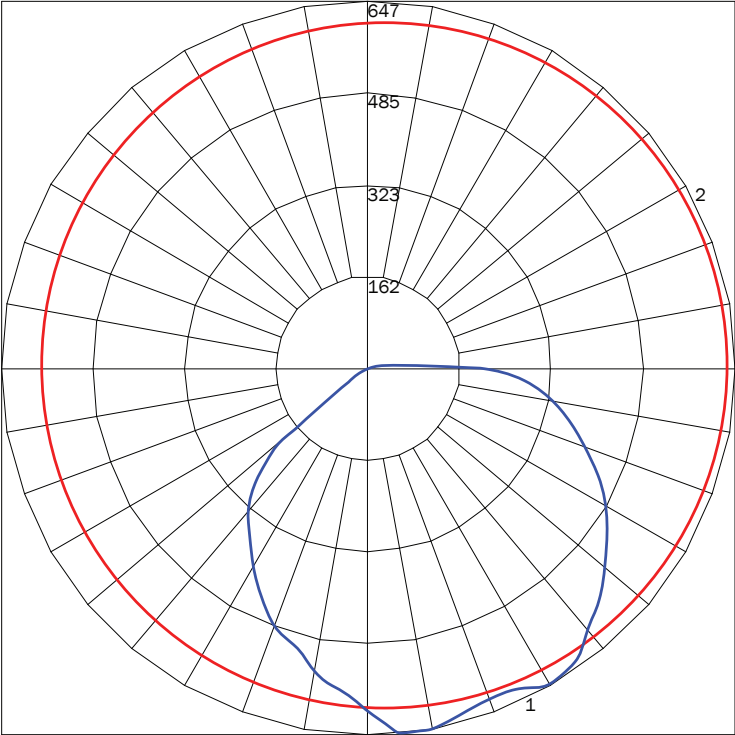
MAXIMUM CANDELA = 646.85 LOCATED AT HORIZONTAL ANGLE = 0, VERTICAL ANGLE = 5 # 1 - VERTICAL PLANE THROUGH HORIZONTAL ANGLES (0 - 180) (THROUGH MAX. CD.) # 2 - HORIZONTAL CONE THROUGH VERTICAL ANGLE (5) (THROUGH MAX. CD.)
