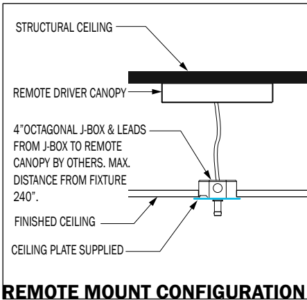
REMOTE MOUNT CONFIGURATION
