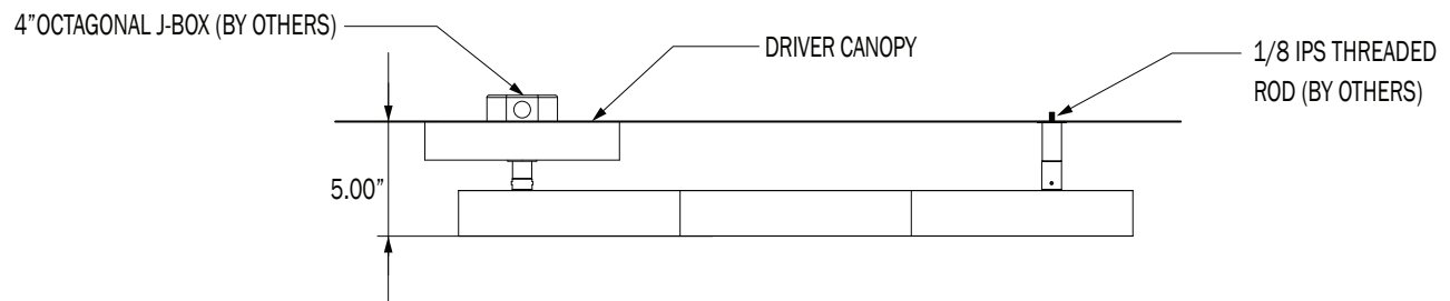
CEILING MOUNT CONFIGURATION
