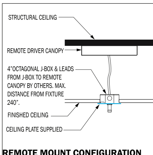
REMOTE MOUNT CONFIGURATION
