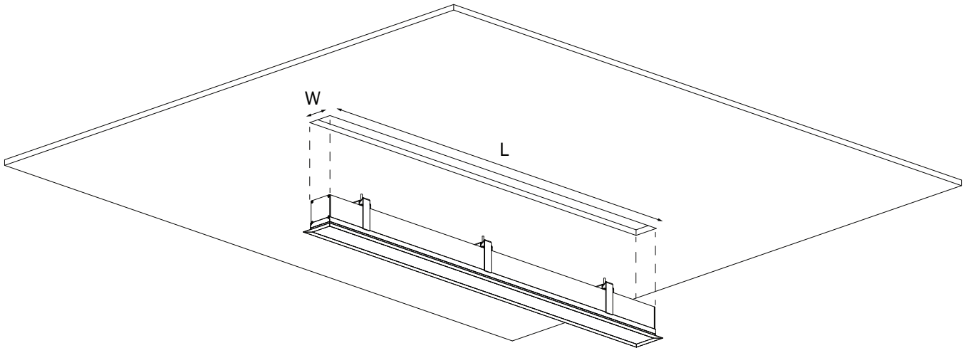
CEILING TRIM CONFIGURATION (TR)
