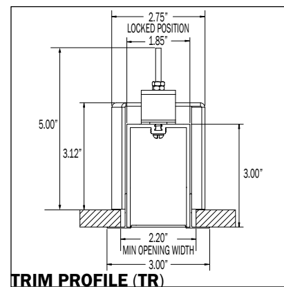
TRIM CONFIGURATION (TR)
