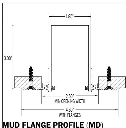
MUD FLANGE CONFIGURATION (MD)
