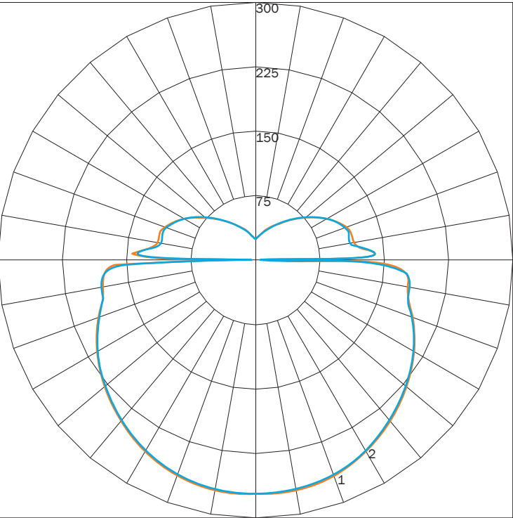
POLAR GRAPH
