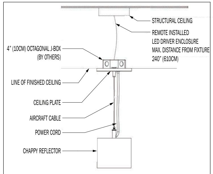
REMOTE DRIVER
