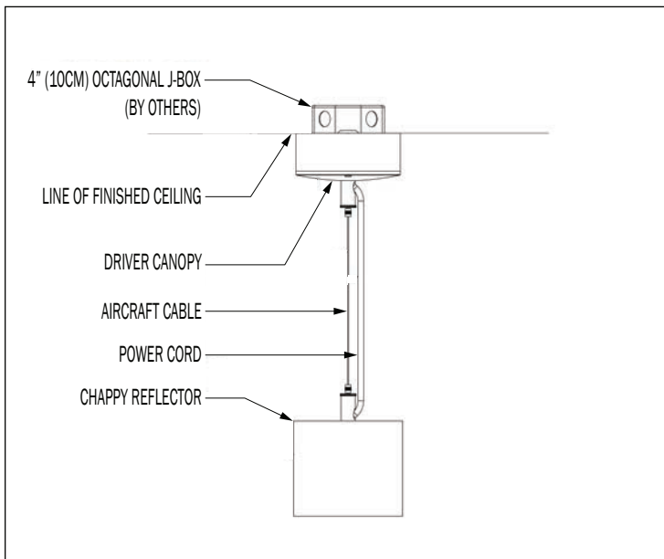
INTEGRAL DRIVER
